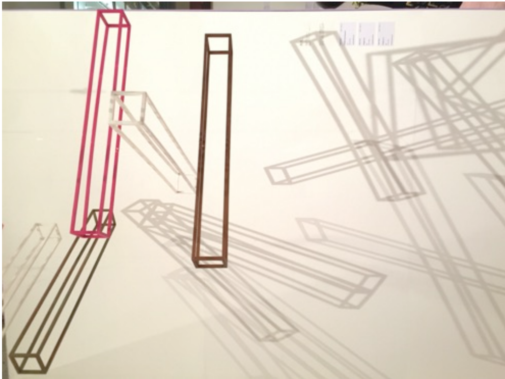
Moving objects light and shadows
